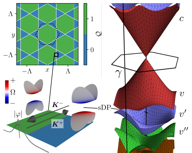
Figure 1. A typical miniband spectrum of graphene encapsulated into mutually aligned hBN crystals. Top inset. Map of locally-defined v -miniband Chern number, Q . Bottom inset. Dispersion and Berry curvature at the v/v' miniband edge in the gaped regions and 1D modes counter-propagating in K^\pm valleys along a Kagomé network of locally gapless v/v' miniband edges.
