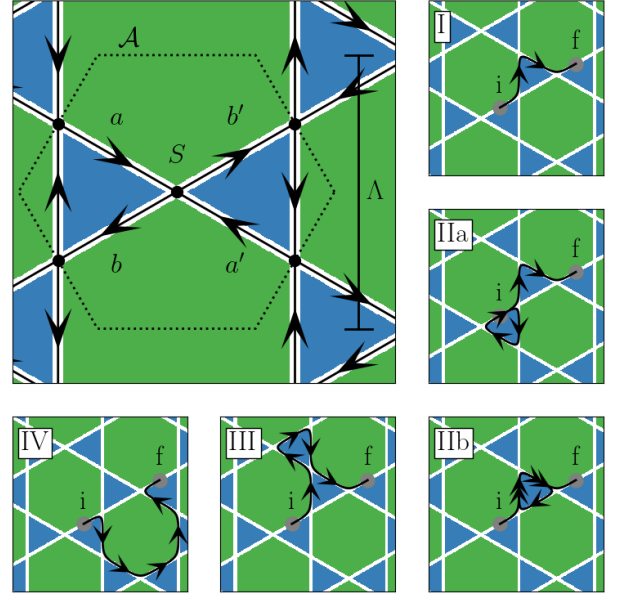
Figure 3. Top left. The hexagonal structural element of the Kagomé network of channels of area \mathcal{A} = \sqrt{3}\Lambda^2/2 and containing one Q = 0 bowtie and one Q = 1 hexagon. The propagation of electrons in the \mathbf{K}_+ valley is shown, scattering at the three nodes. Clockwise from top right. The five shortest paths for an electron wave packet to propagate from an injection position “i” to “f” (double arrows indicate a channel is traversed twice).
